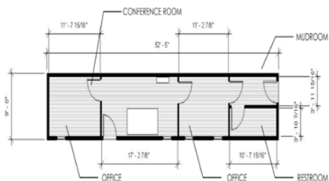
Layout for Mobile Command Post Trailer
